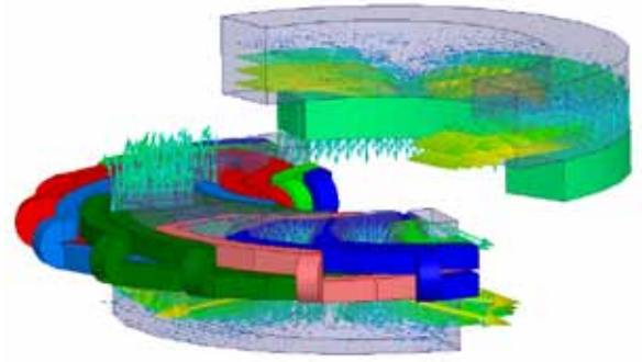
Axial magnetic field distribution on axial permanent magnet machine
