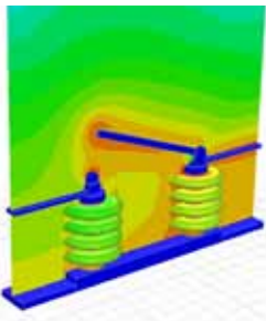
Maxwell-simulated electromagnetic field distribution on transformer terminals
