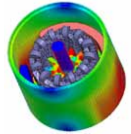
DC permanent magnet motor solved by Maxwell with ANSYS RMxprt
